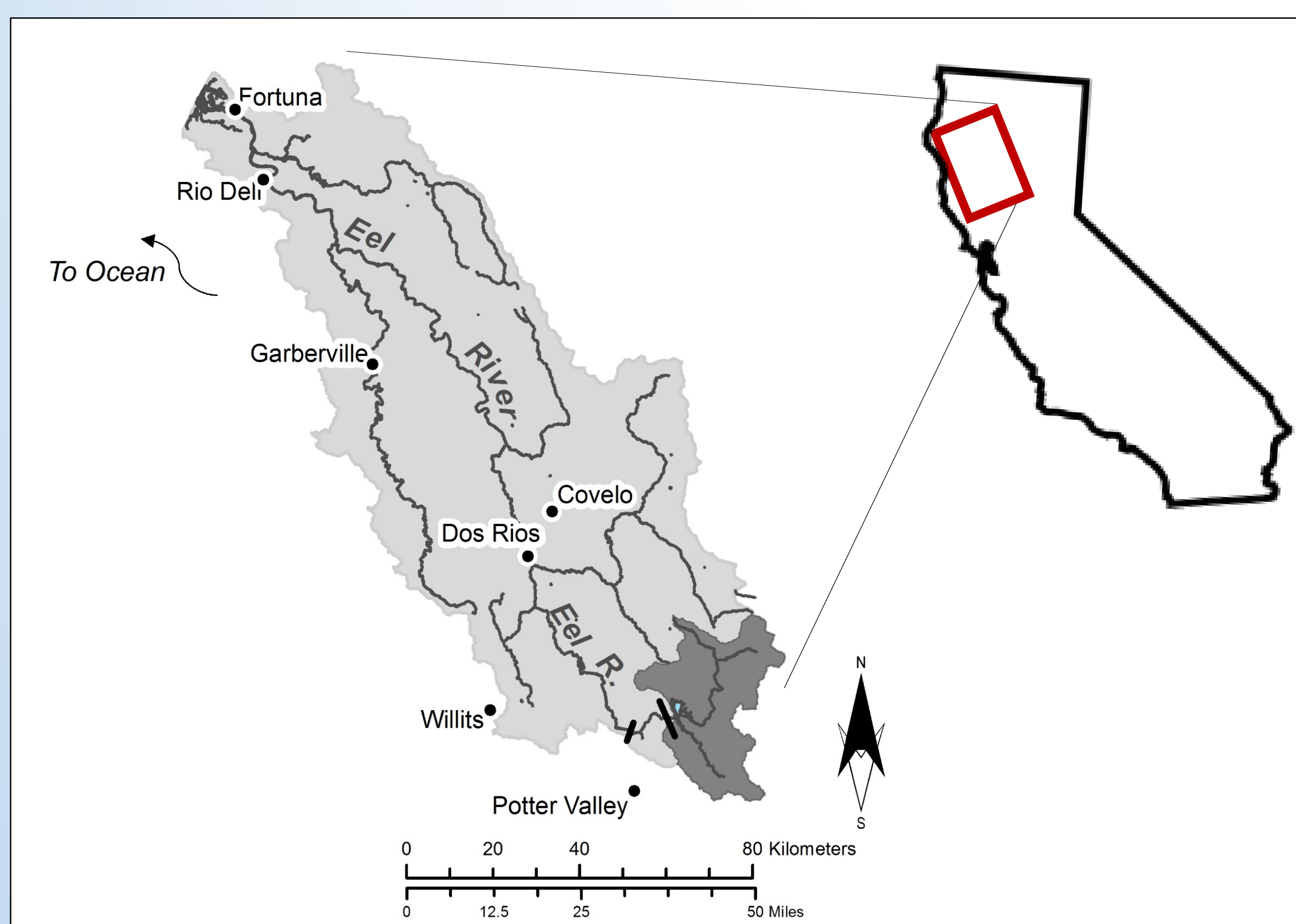
Figure 1. The Eel River watershed is located in northwestern California. Along the mainstem Eel River are two dams (black lines), and the study area is located upstream of Scott Dam (shaded in dark gray).
