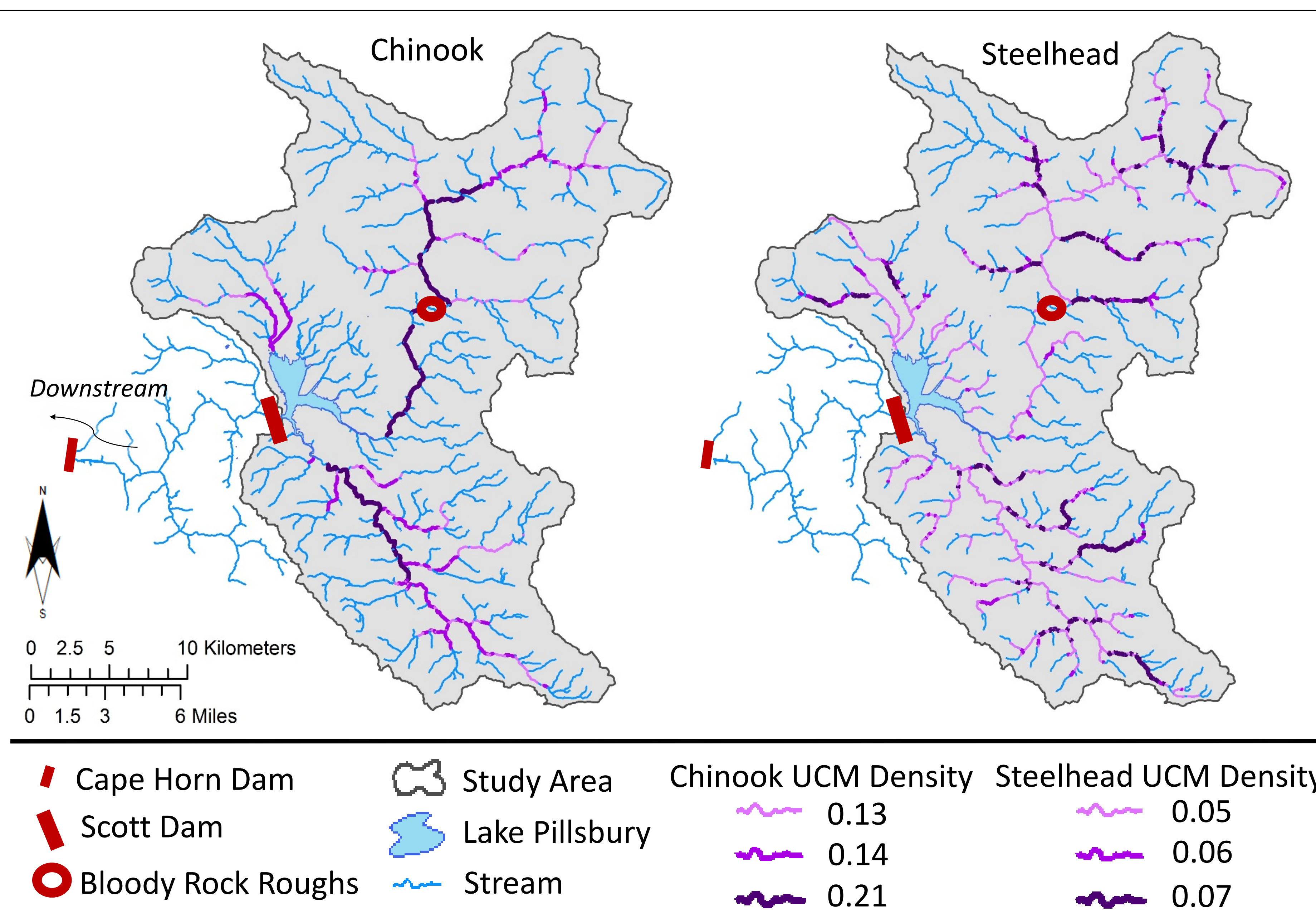
Figure 5. Potential distribution and juvenile densities among stratified reaches in the waterways upstream of Scott Dam for Chinook salmon (left) and steelhead trout (right).
