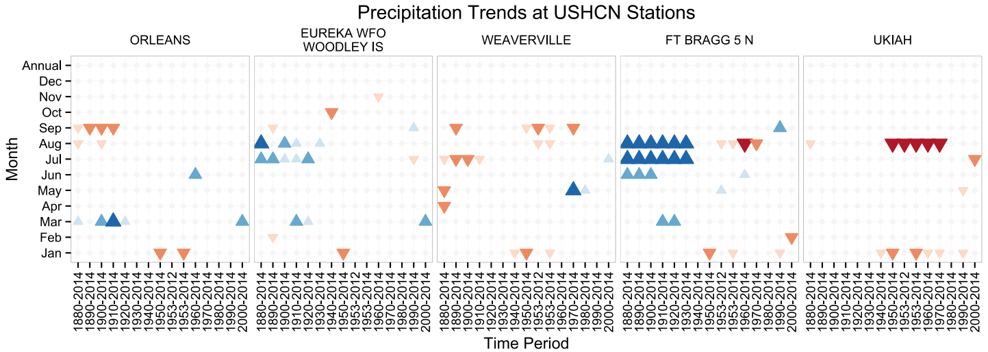
Figure 8. Summary of Mann-Kendall trend tests for monthly and annual precipitation at U.S. Historical Climatology Network (USHCN) stations near the Eel River Basin, for multiple time periods ending in 2014, as well as 1953-2012 (the period evaluated by Asarian and Walker in press ).
